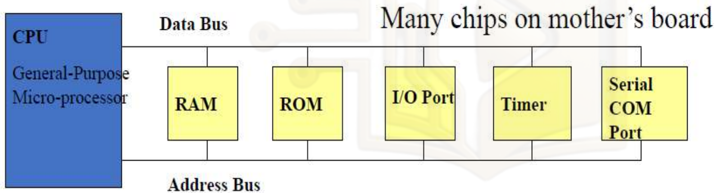
General-Purpose Microprocessor System
